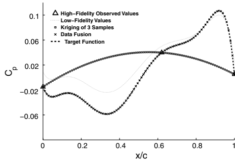
Fig. 3 Cokriging approximation of the aerofoil pressure distribution based on many cheap samples and three expensive samples.
