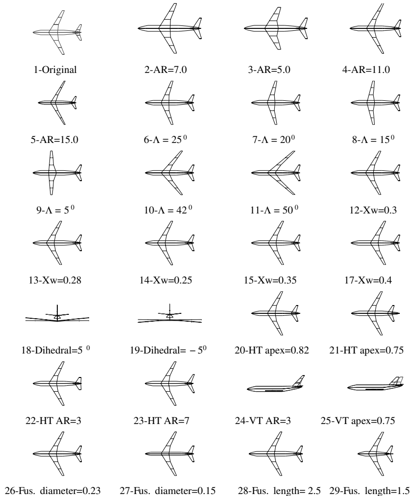
Fig. 8 Geometry increments used to test the data fusion approach. AR: aspect ratio; \Lambda : wing sweep; X_w : location of the wing down the fuselage; Dihedral: dihedral of the wing; VT AR: aspect ratio of the vertical tail; VT apex: apex of the vertical tail; HT AR: aspect ratio of the horizontal tail; HT apex: apex of the horizontal tail; Fus. diameter: diameter of fuselage; Fus. length: fuselage length. Note that in cases 18, 19, 24, and 25 the outline of the original geometry is included to emphasize the geometry increment involved.
